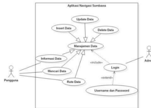
Gambar 2.9 Use Case Diagram
