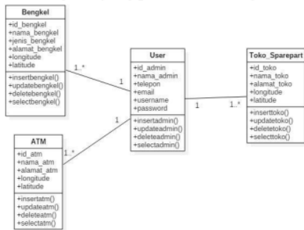
Gambar 2.6 Class Diagram
