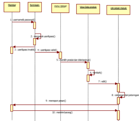
Gambar 6. Sequence diagram
