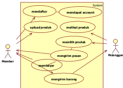
Gambar 5. Usecase Diagram
