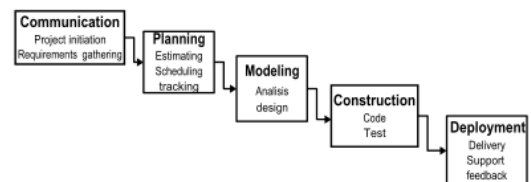
Gambar 1. Waterfall model
