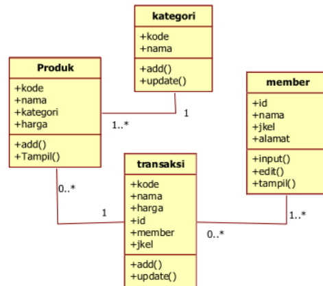
Gambar 6. Calss diagram
