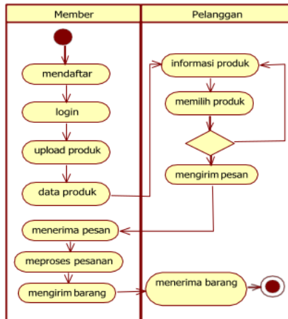
Gambar 7. Activity diagram
