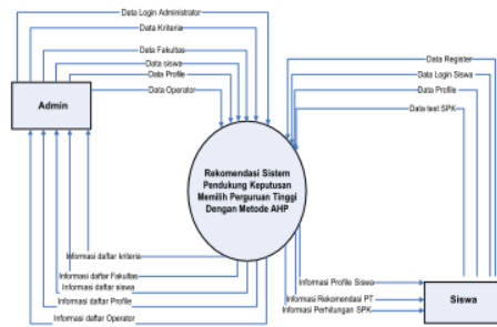
Gambar 2.4 Diagram Context
