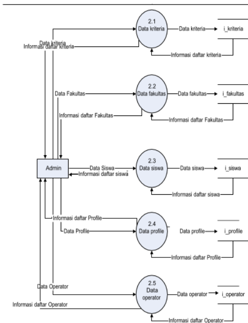
Gambar 2.6 Diagram Level 2
