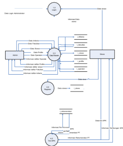
Gambar 2.5 Diagram Level 1
