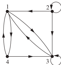
FIGURE 5 The directed graph of the relation R_2 .
