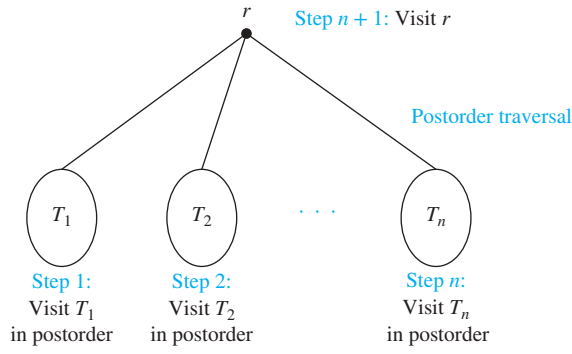
FIGURE 7 Postorder traversal.
