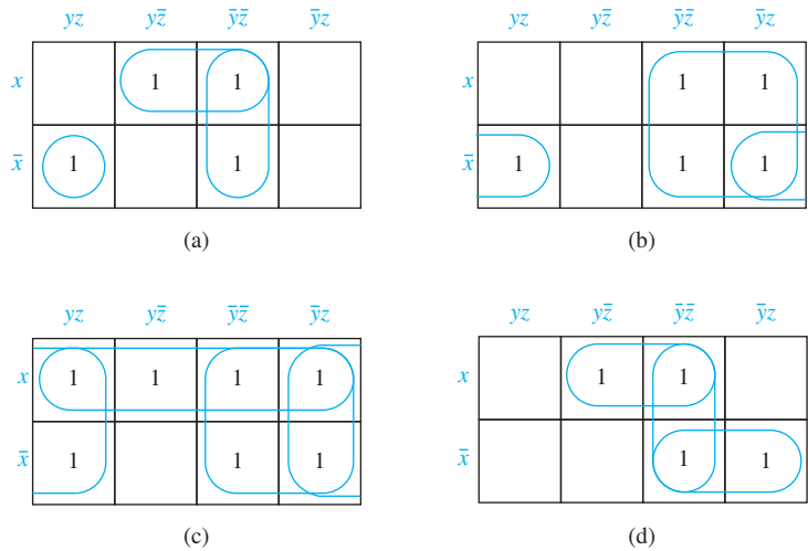
FIGURE 7 Using K-maps in three variables.
