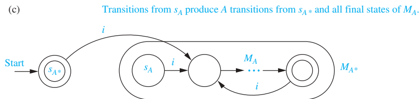
FIGURE 2 Building automata to recognize concatenations, unions, and Kleene closures.
