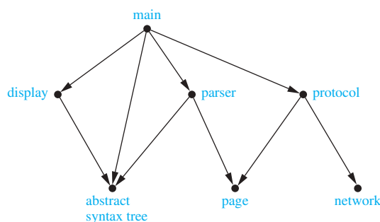
FIGURE 9 A module dependency graph.
