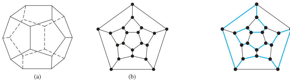
FIGURE 9 A solution to the "A Voyage Round the World" puzzle.
