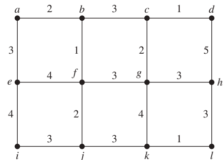
FIGURE 3 A weighted graph.
