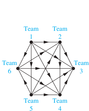
FIGURE 14 A graph model of a round-robin tournament.
