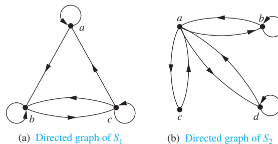
FIGURE 6 The directed graphs of the relations S_1 and S_2 .
