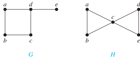
FIGURE 11 Two graphs that do not have a Hamiltonian circuit.
