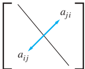
FIGURE 2 \mathbf{A} symmetric matrix.
