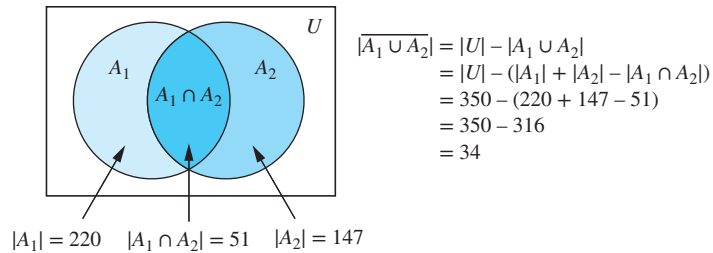
FIGURE 3 Applicants who majored in neither computer science nor business.
