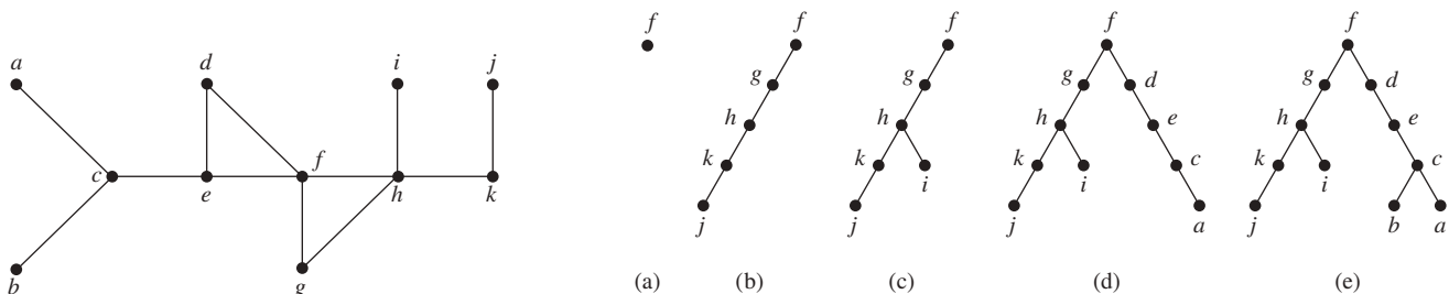
FIGURE 6 The graph G .
