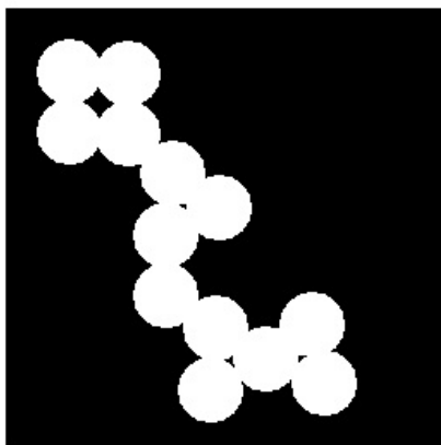
Source Image
