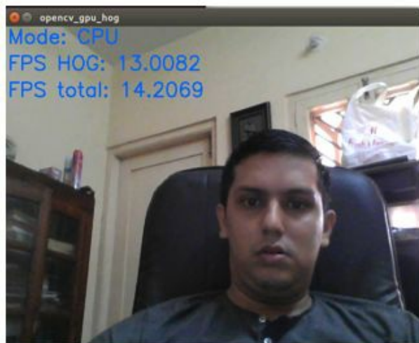
CPU Performance
