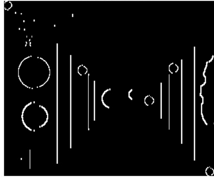
Scharr-xy derivative
