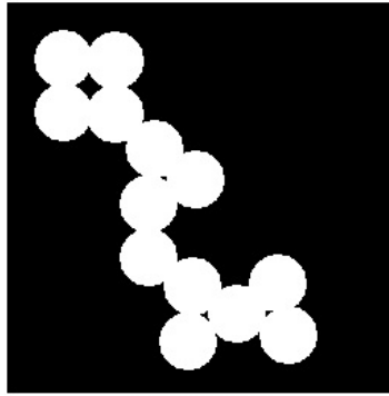
Source Image
