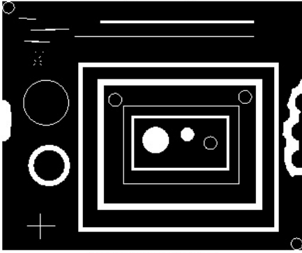
Scharr-y derivative
