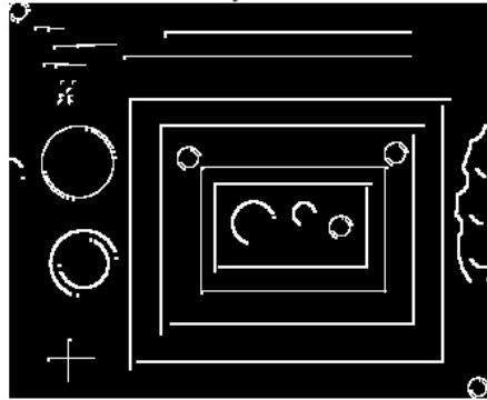
Scharr-xy derivative
