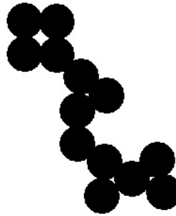
Inverted Image
