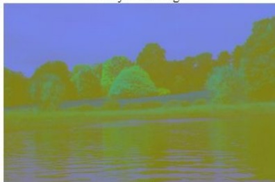
YCrCb Image
