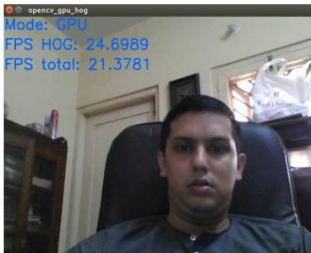
GPU Performance
