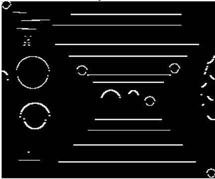
Scharr-y derivative
