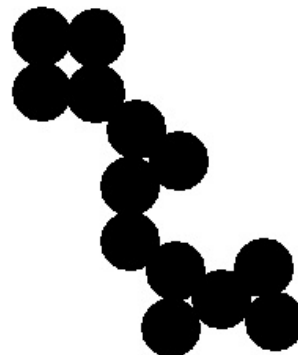
Inverted Image
