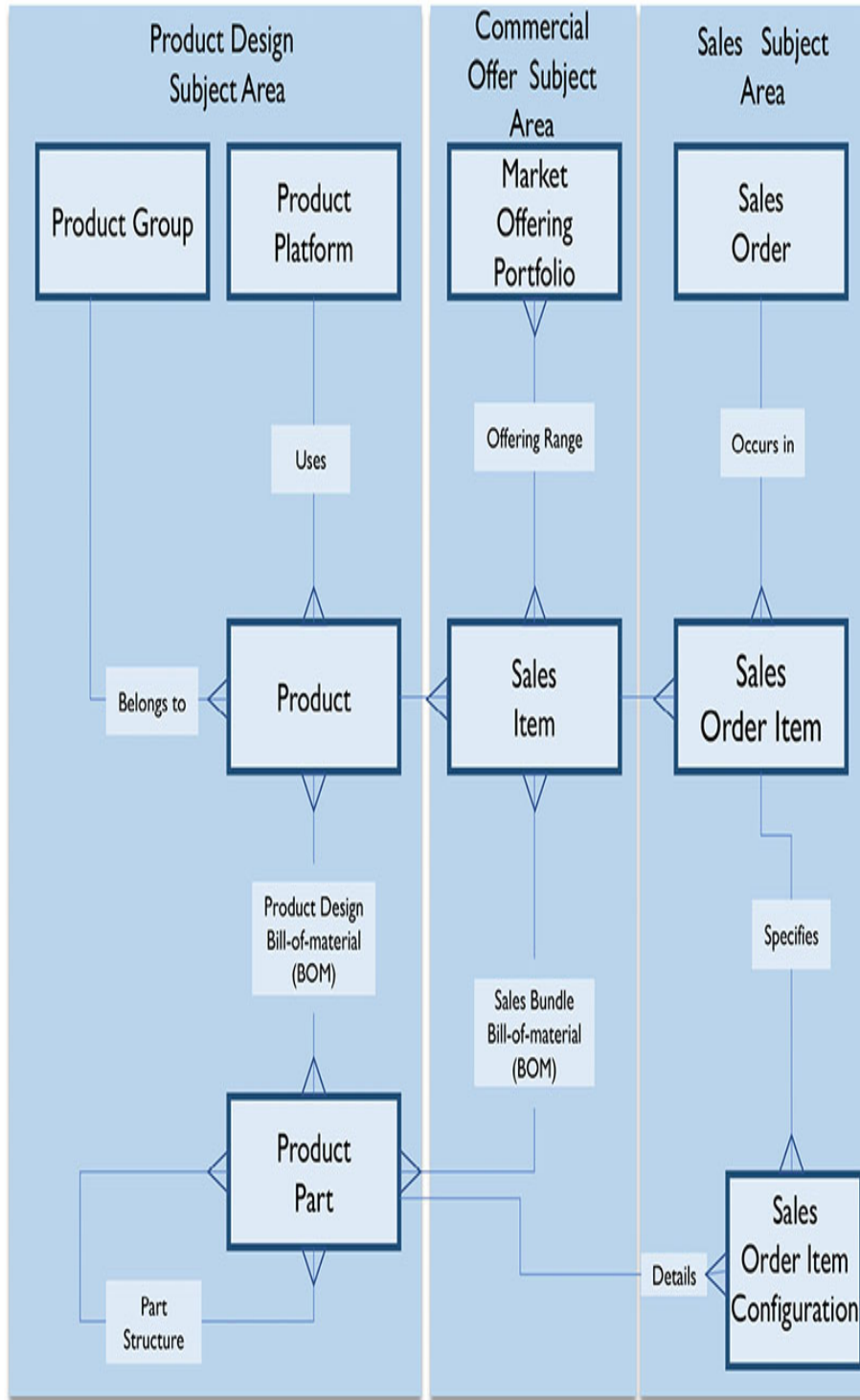
Figure 24 Subject Area Models Diagram Example
