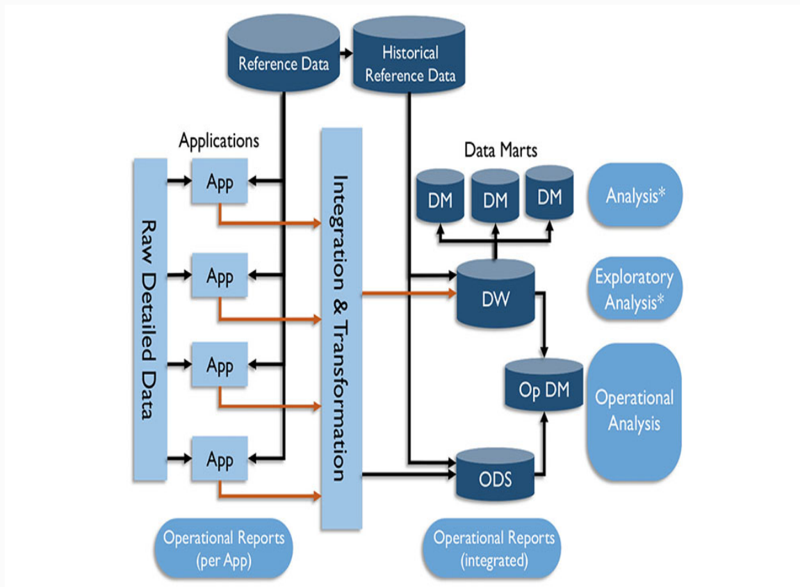
Figure 80 The Corporate Information Factory
