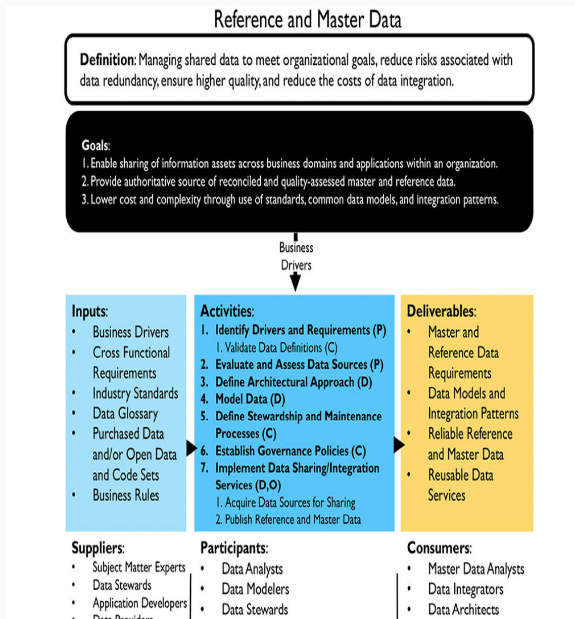
Figure 75 Context Diagram: Reference and Master Data
