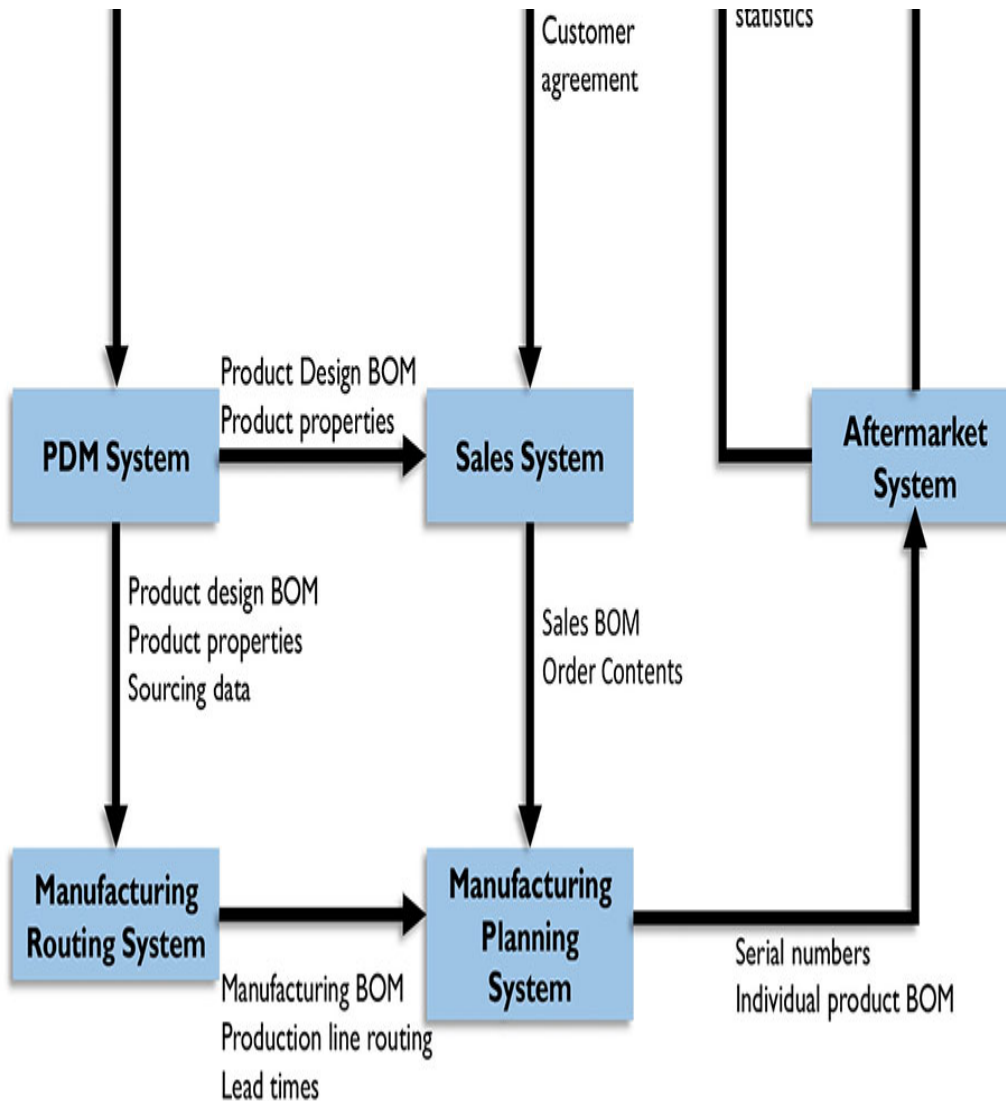
Figure 26 Data Flow Diagram Example
