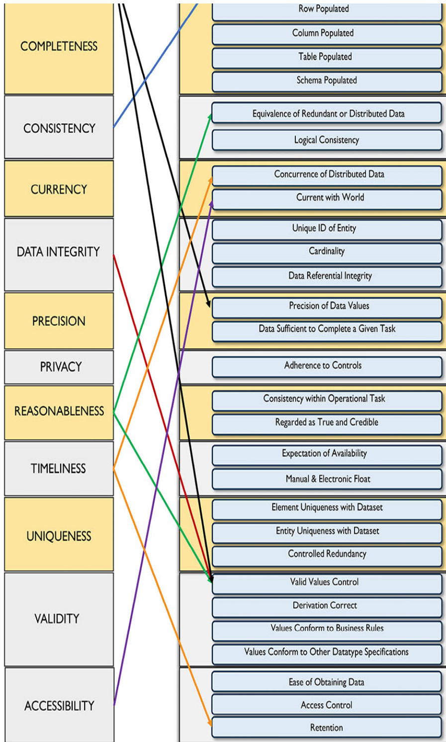
Figure 92 Relationship Between Data Quality Dimensions 77
