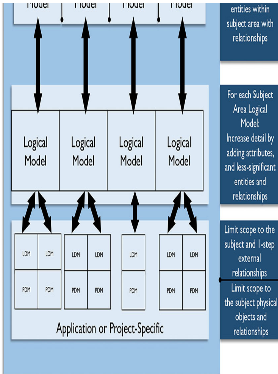
Figure 23 Enterprise Data Model
