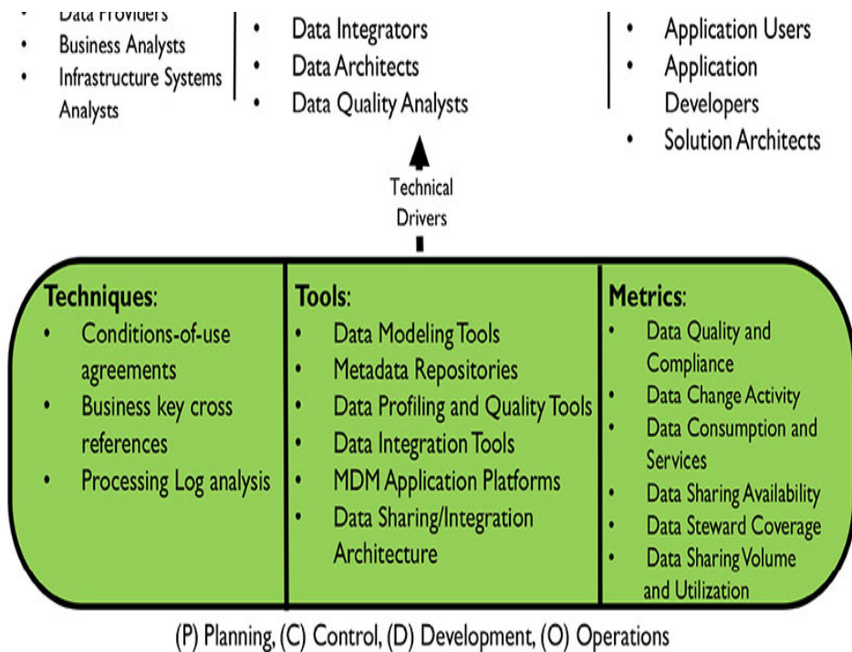
Figure 75 Context Diagram: Reference and Master Data
