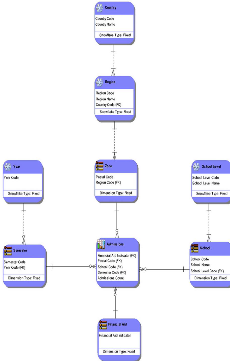
Figure 49 Dimensional Logical Data Model
