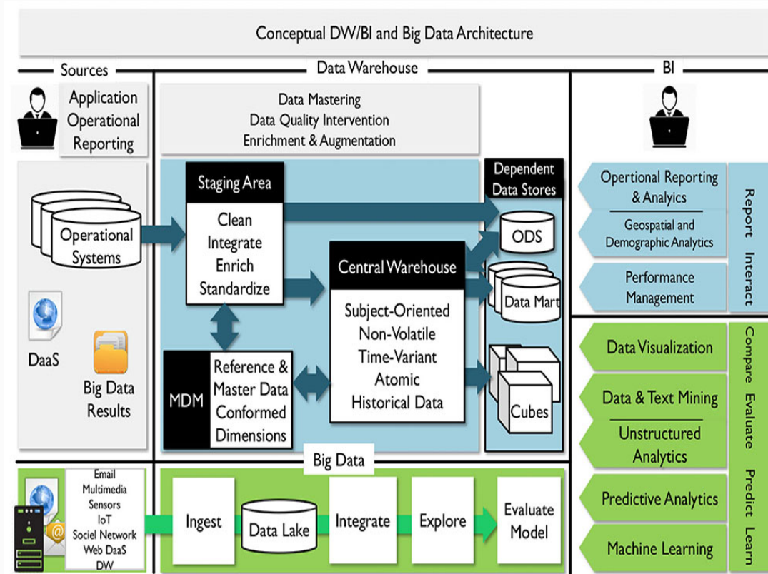
Figure 100 Conceptual DW/BI and Big Data Architecture
