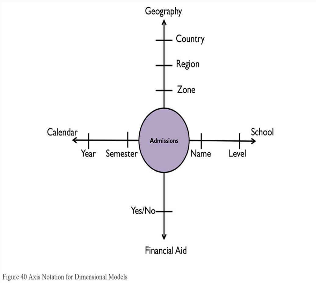
Figure 40 Axis Notation for Dimensional Models
