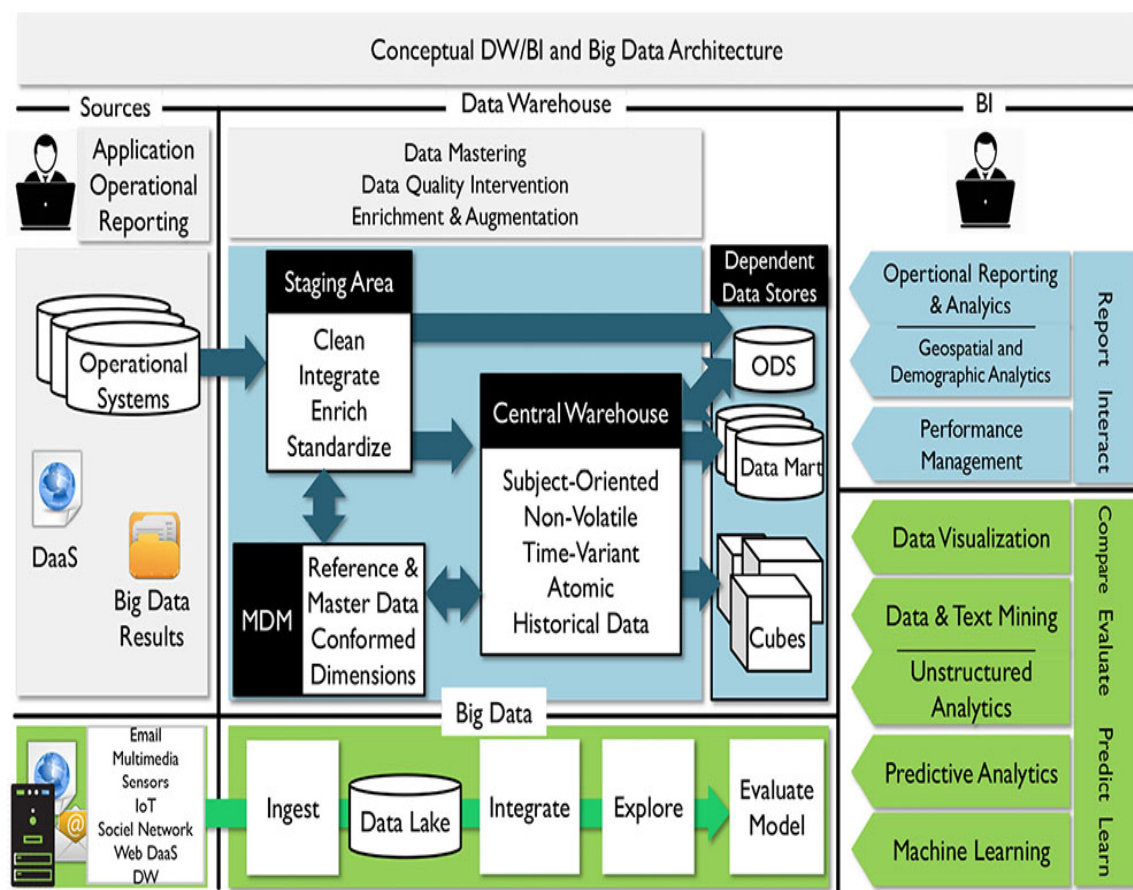
Figure 82 Conceptual DW/BI and Big Data Architecture
