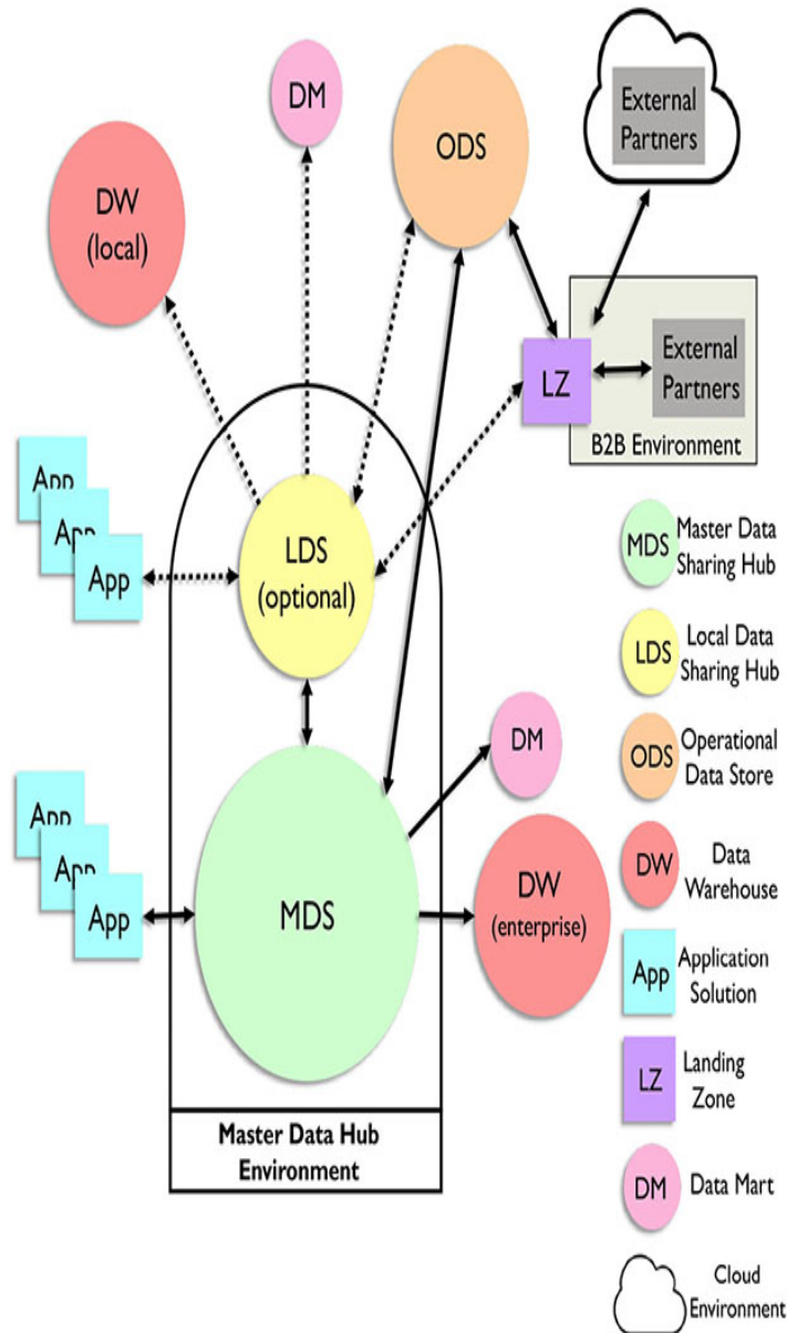
Figure 77 Master Data Sharing Architecture Example
