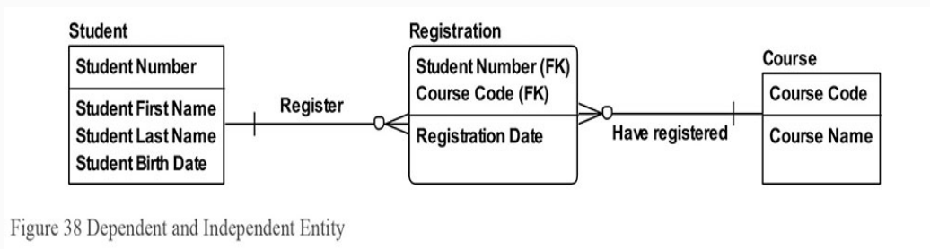
Figure 38 Dependent and Independent Entity
