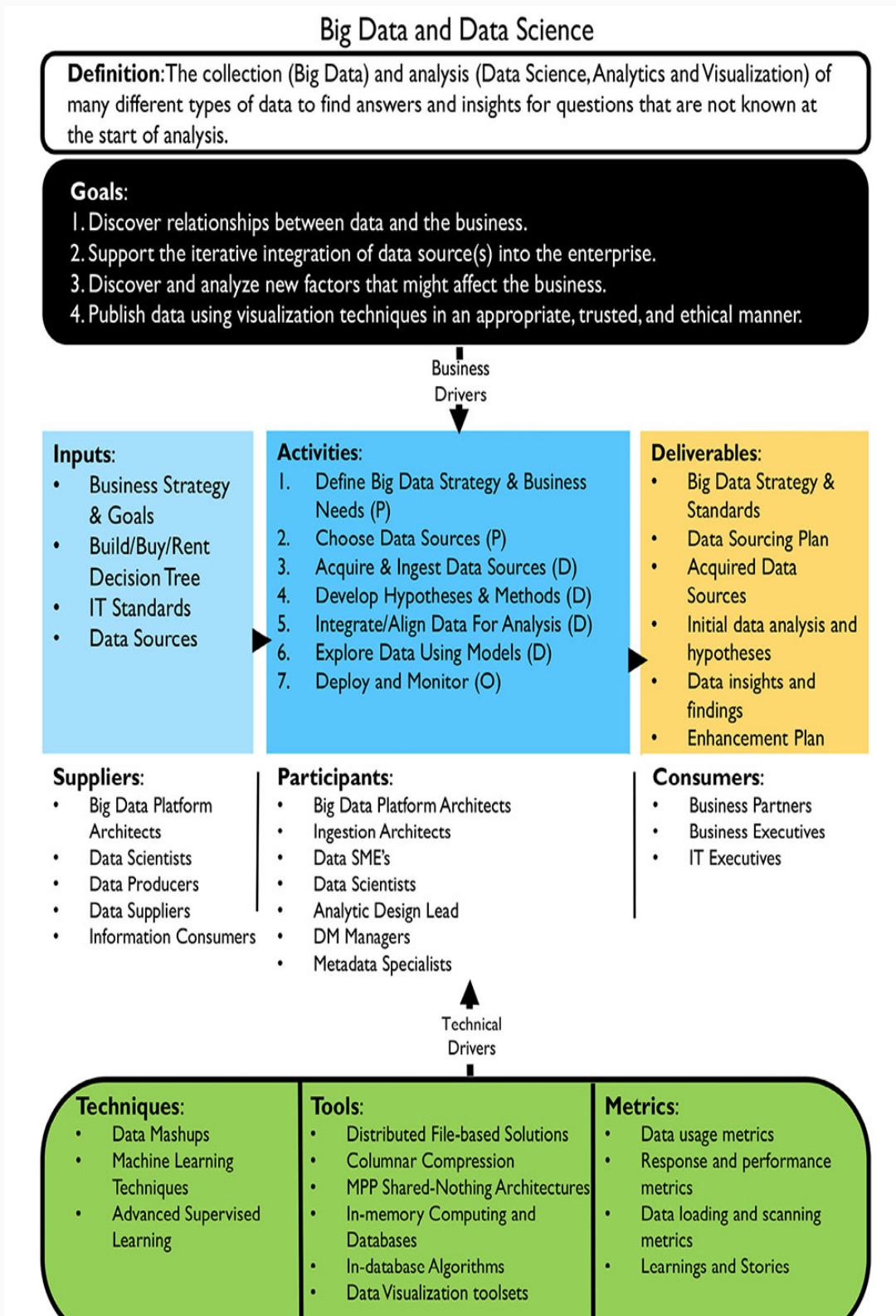
Figure 97 Context Diagram: Big Data and Data Science
