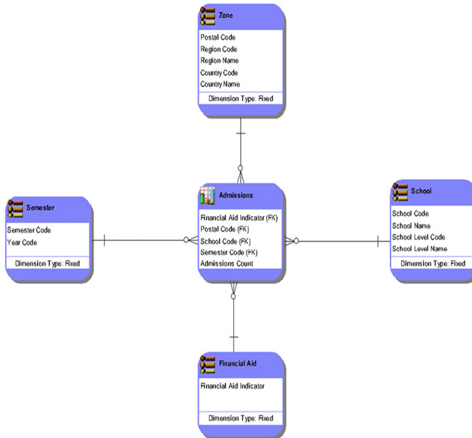
Figure 51 Dimensional Physical Data Model
