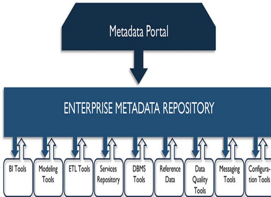
Figure 85 Centralized Metadata Architecture
