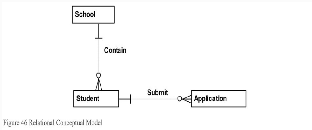
Figure 46 Relational Conceptual Model
