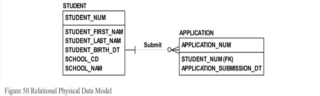
Figure 50 Relational Physical Data Model
