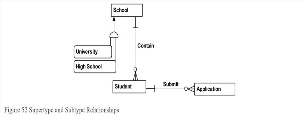
Figure 52. Supertype and Subtype Relationships
