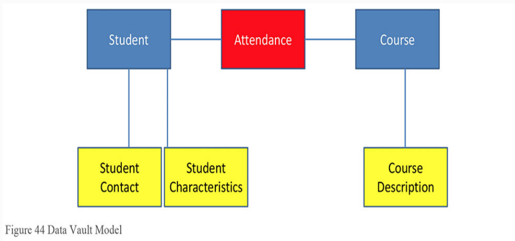
Figure 44 Data Vault Model
