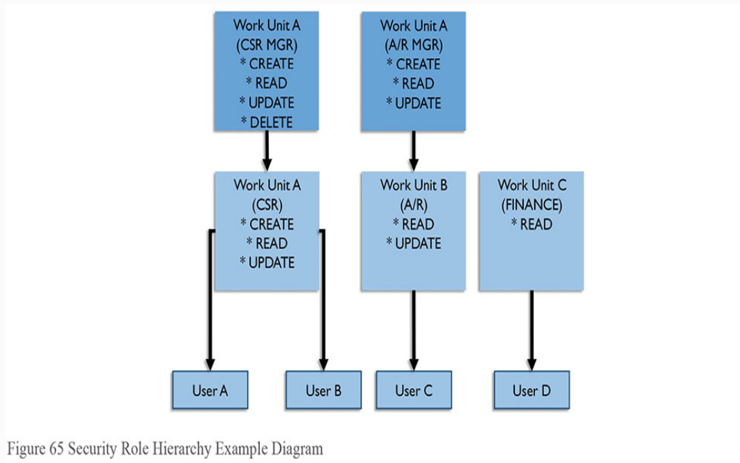
Figure 65 Security Role Hierarchy Example Diagram
