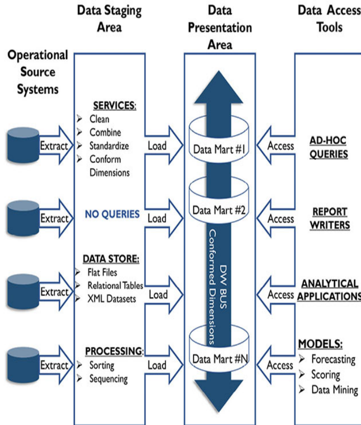
Figure 81 Kimball's Data Warehouse Chess Pieces 67
