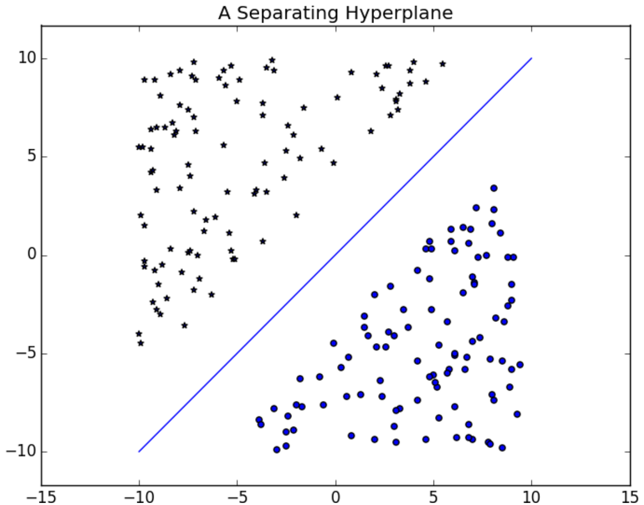
Figure 16-6. A separating hyperplane
