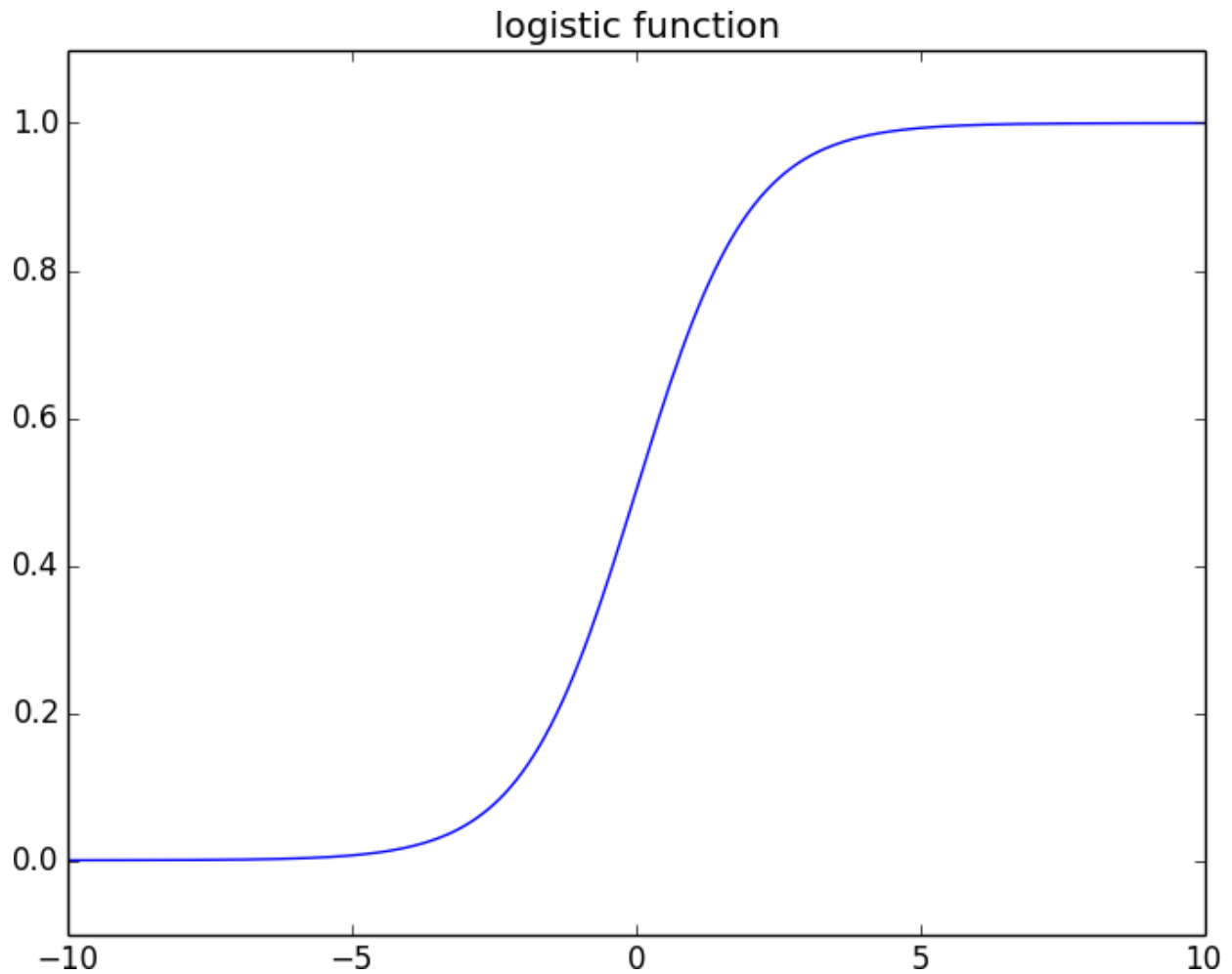
Figure 16-3. The logistic function
