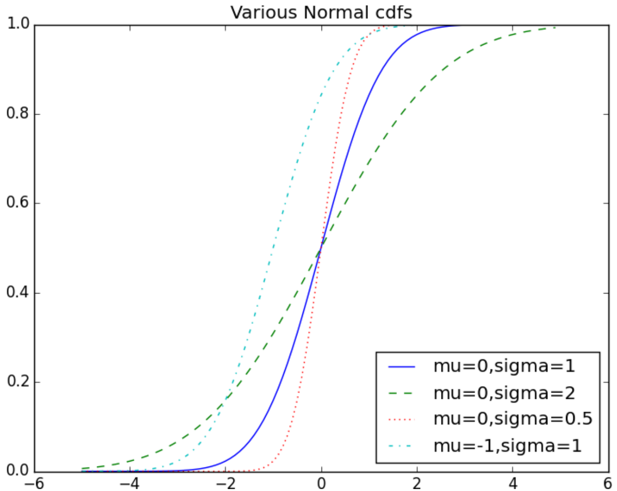
Figure 6-3. Various normal CDFs
