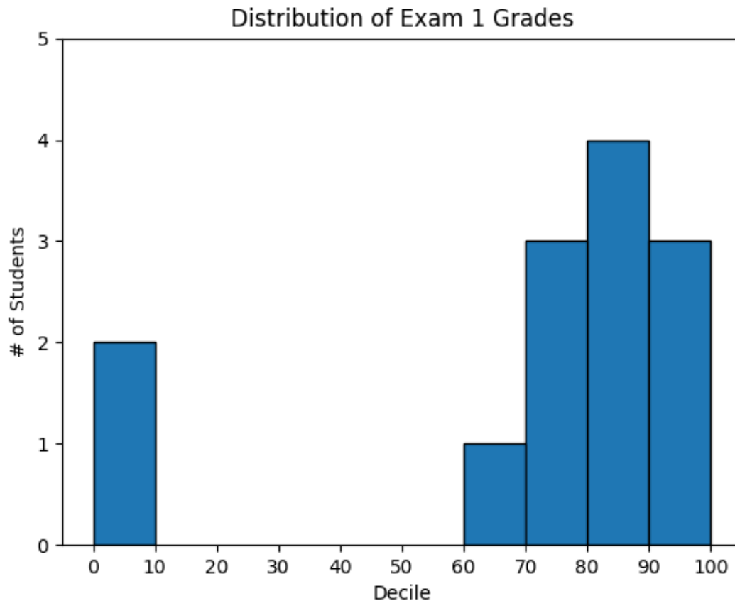
Figure 3-3. Using a bar chart for a histogram
