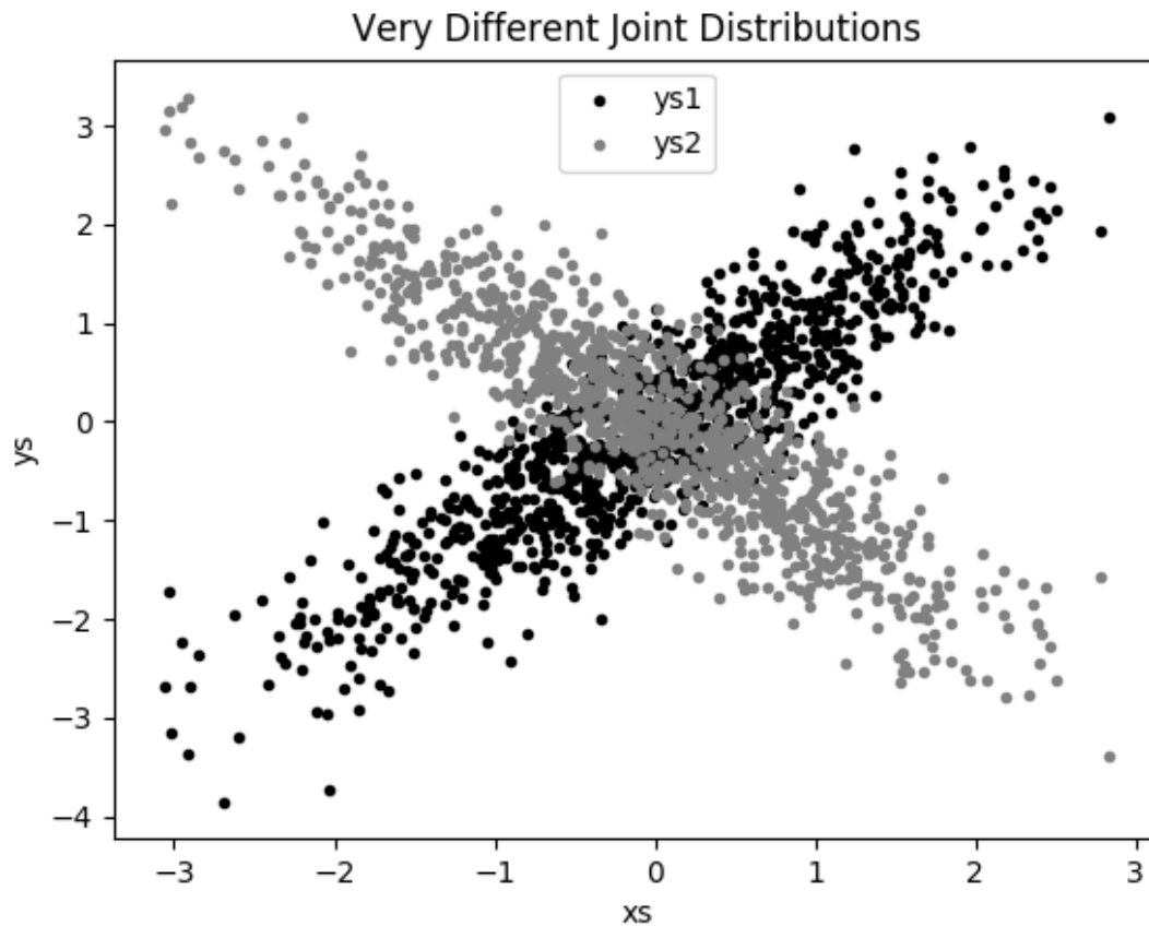
Figure 10-3. Scattering two different ys
