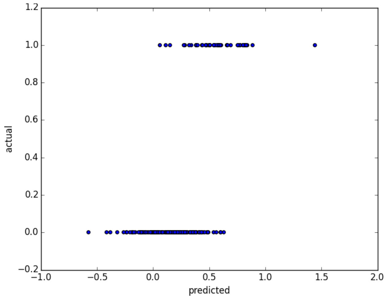
Figure 16-2. Using linear regression to predict premium accounts
