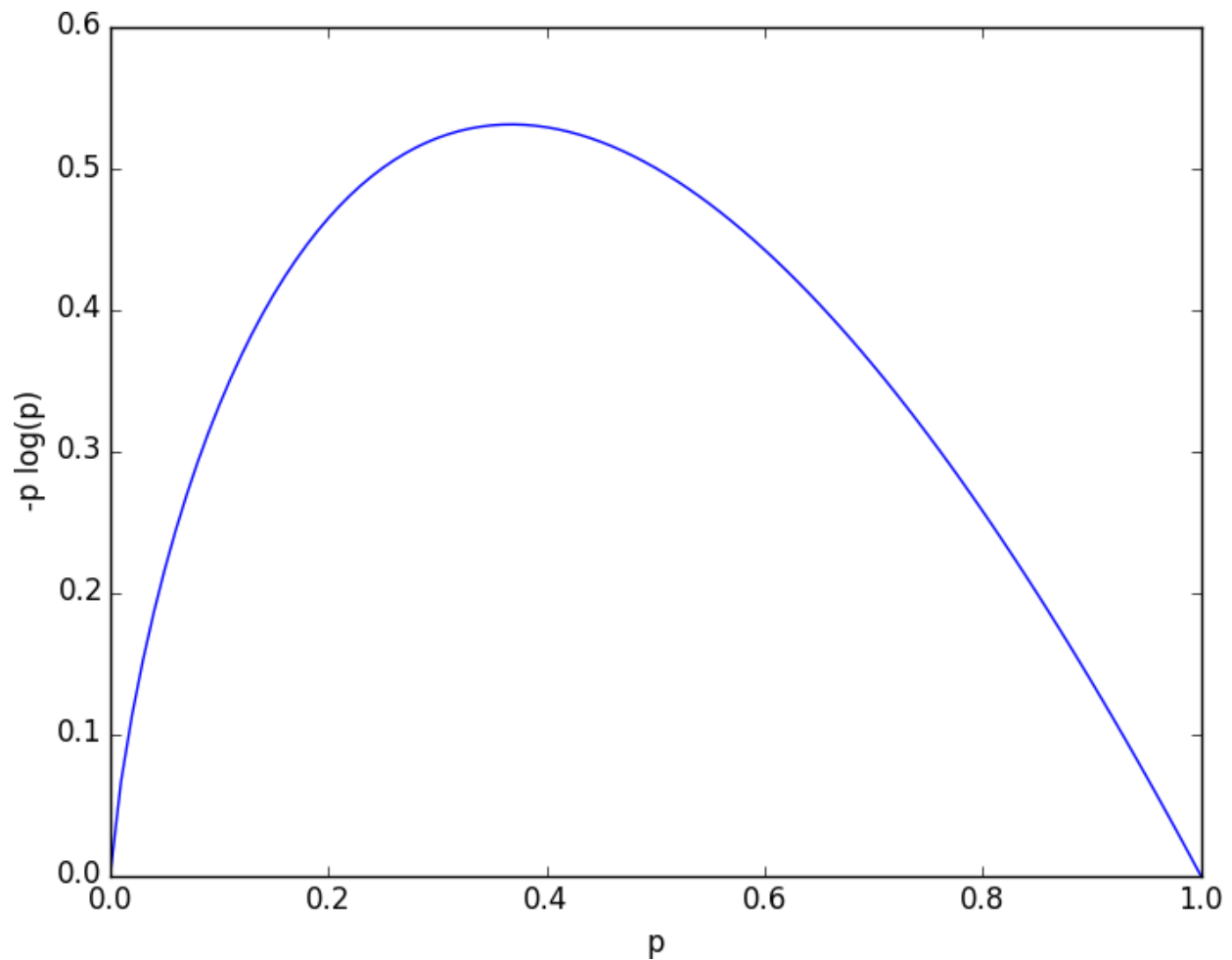
Figure 17-2. A graph of -p \log p
