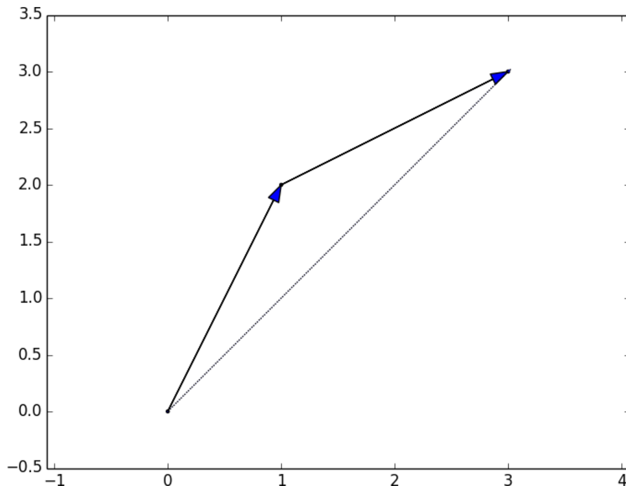
Figure 4-1. Adding two vectors
