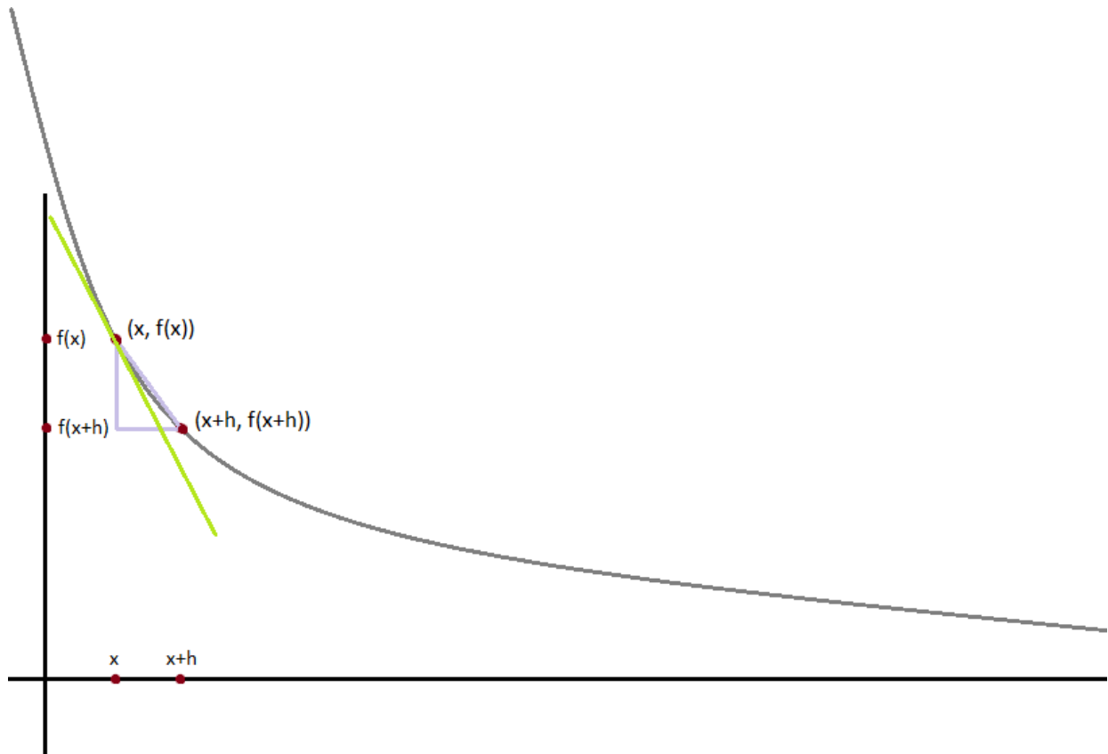
Figure 8-2. Approximating a derivative with a difference quotient
