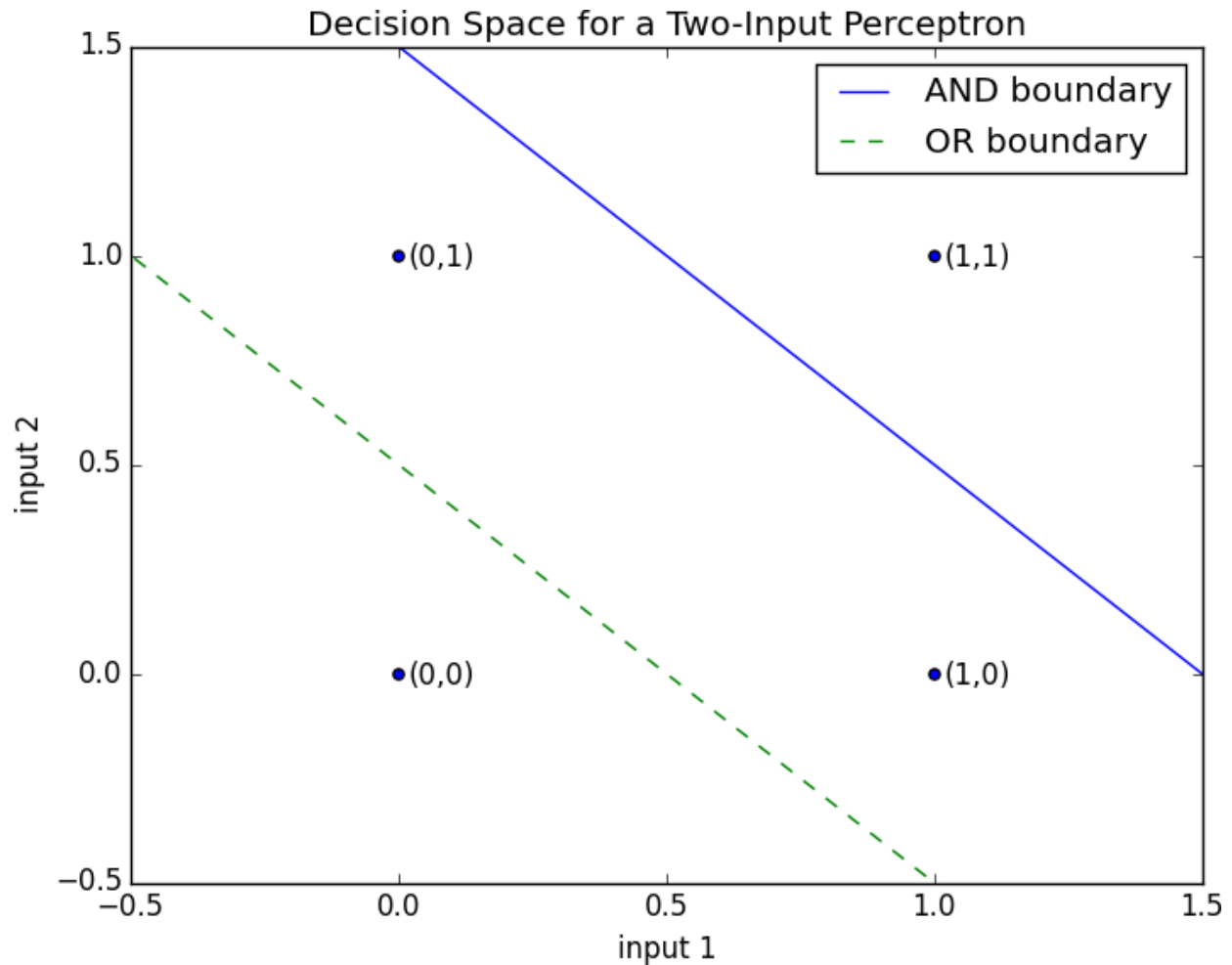
Figure 18-1. Decision space for a two-input perceptron
