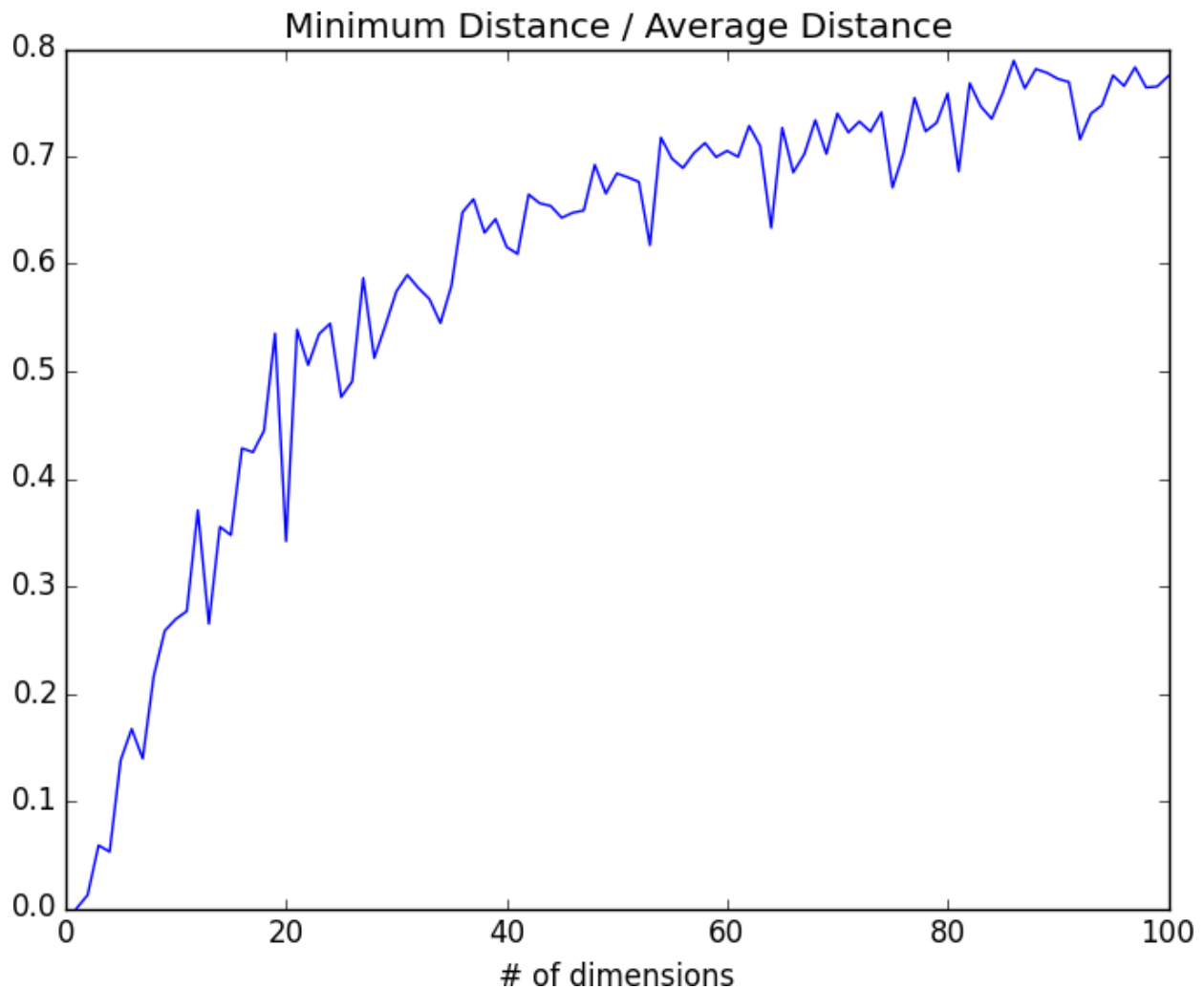
Figure 12-3. The curse of dimensionality again
