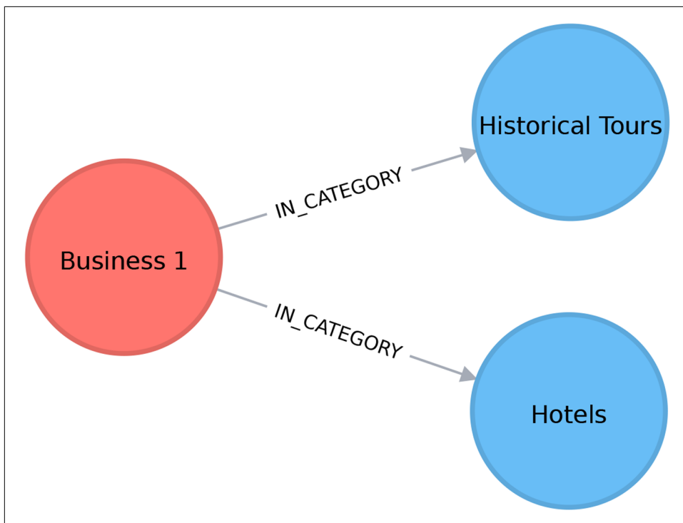
Figure 7-8. A business with two categories
