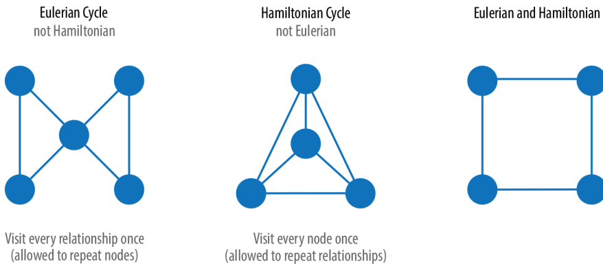
Figure 4-5. Eulerian and Hamiltonian cycles have a special historical significance.
