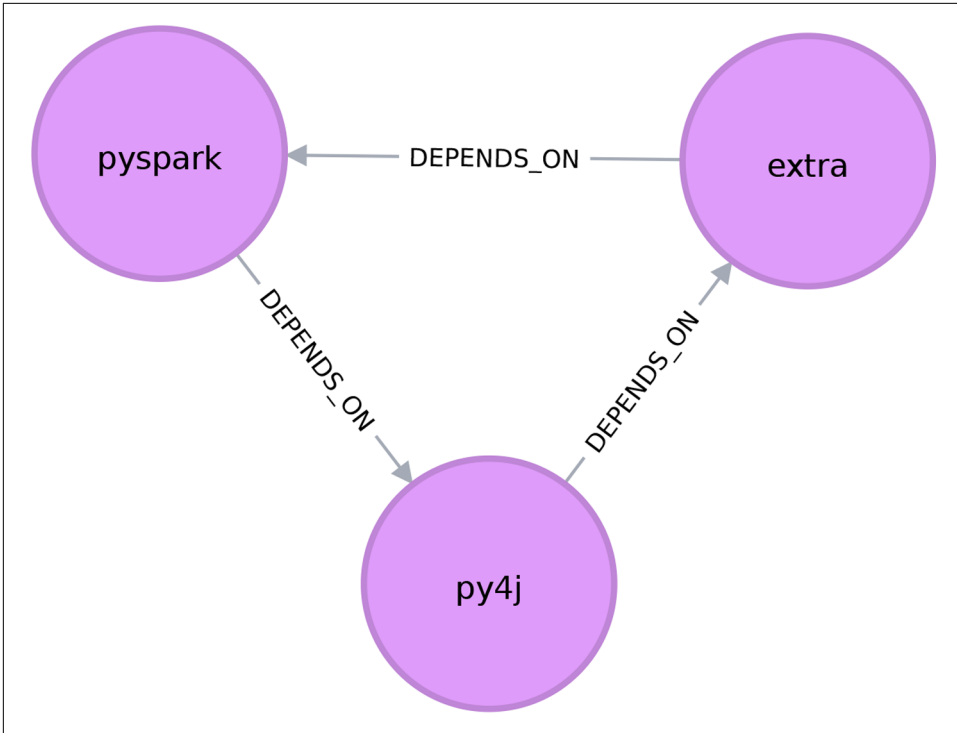
Figure 6-6. A circular dependency between pyspark , py4j , and extra
