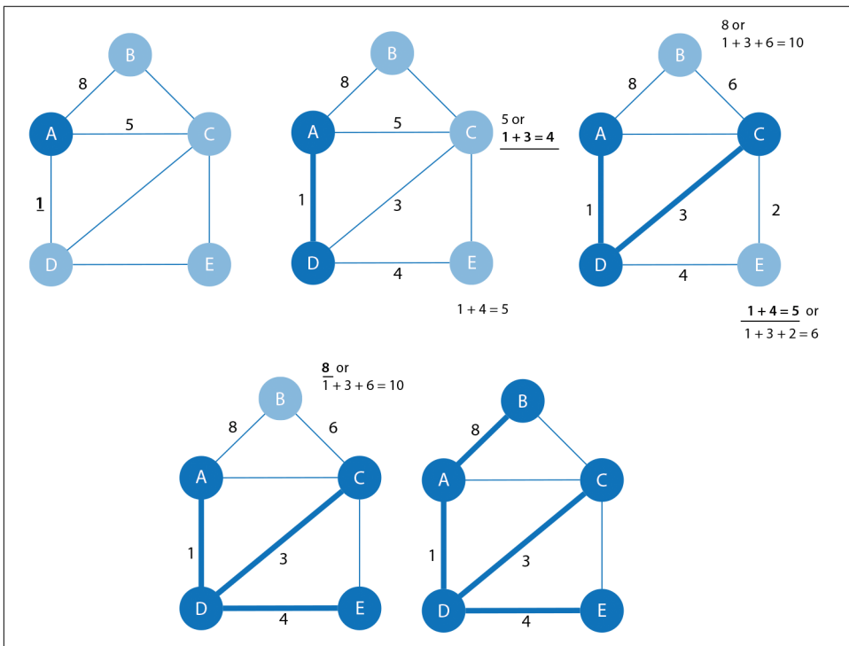
Figure 4-9. The steps of the Single Source Shortest Path algorithm
