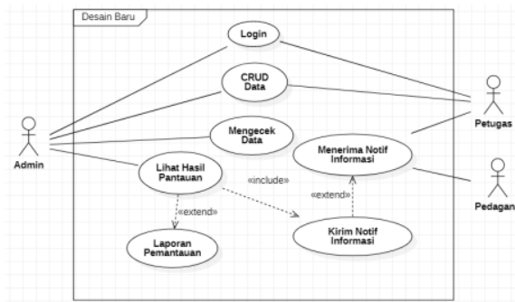
Gambar 2. Tampilan Use Case Diagram
