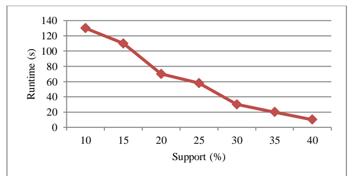
Figure 2 Testing Results of Dataset Connect and Mushroom With Bi-Eclat
