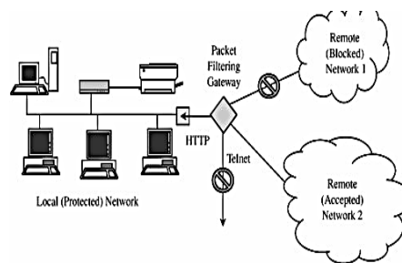
Figure 1. Packet Filter Blocking Address and Protocols
