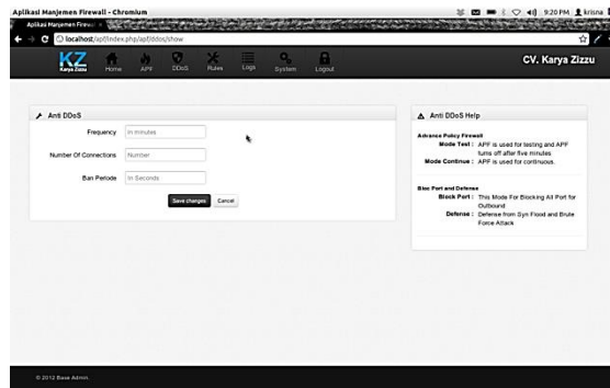
Figure 9. DDoS Menu
