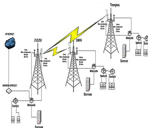
Figure 5. Network Topology
