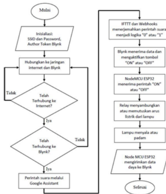
Gambar 4. Flowchart sistem kontrol lampu berbasis IoT
