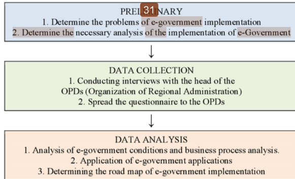
Figure 1. Research Flow
