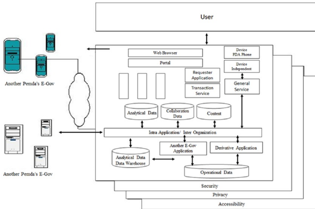
Figure 9. Model interoperability
