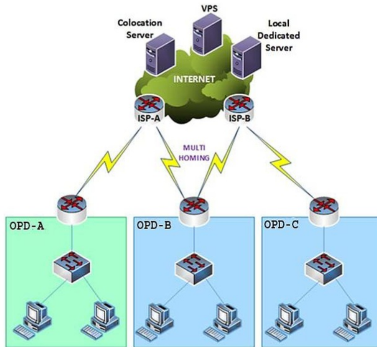
Figure 6. OPD Internet Connection
