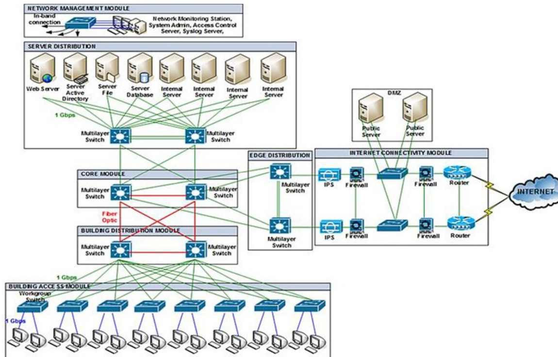
Figure 8. DISKOMINFO LAN Architecture
