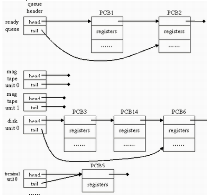
Gambar 4.4. Device Queue.
