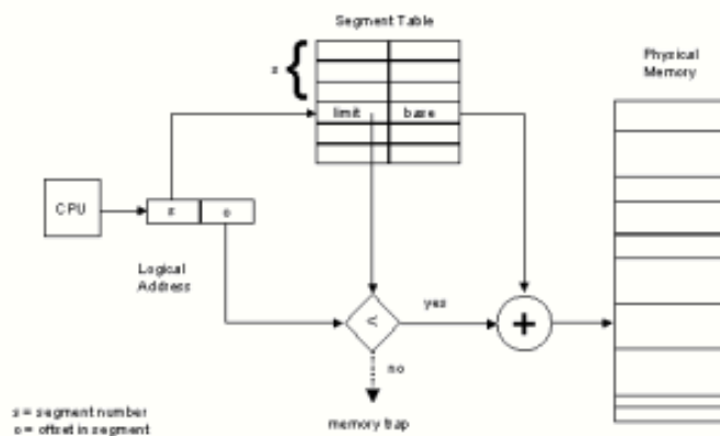
Gambar 6.8. Alamat Logis
