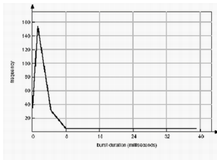
Gambar 5.1. CPU Burst
