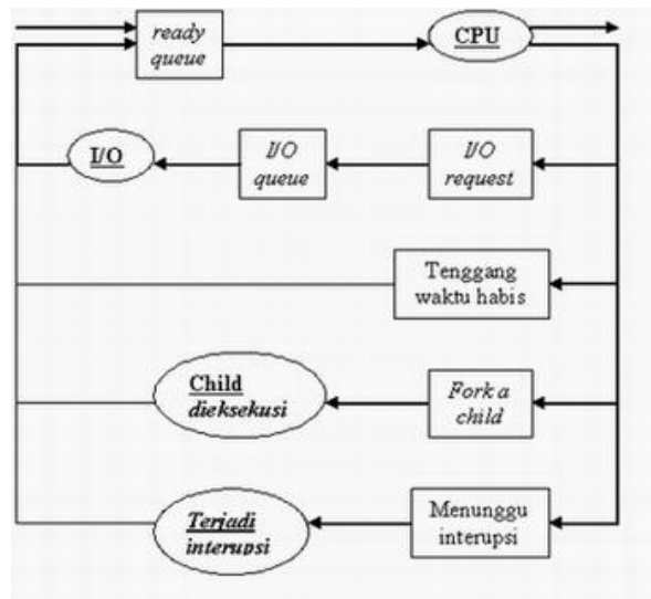
Gambar 4.5. Diagram Antrian.
